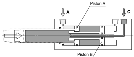
Second-stage retraction
