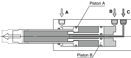
Second-stage extension
