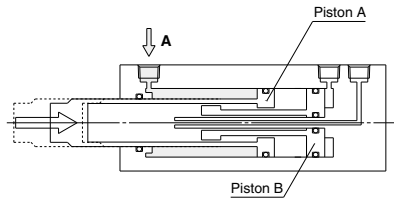
First-stage retraction
